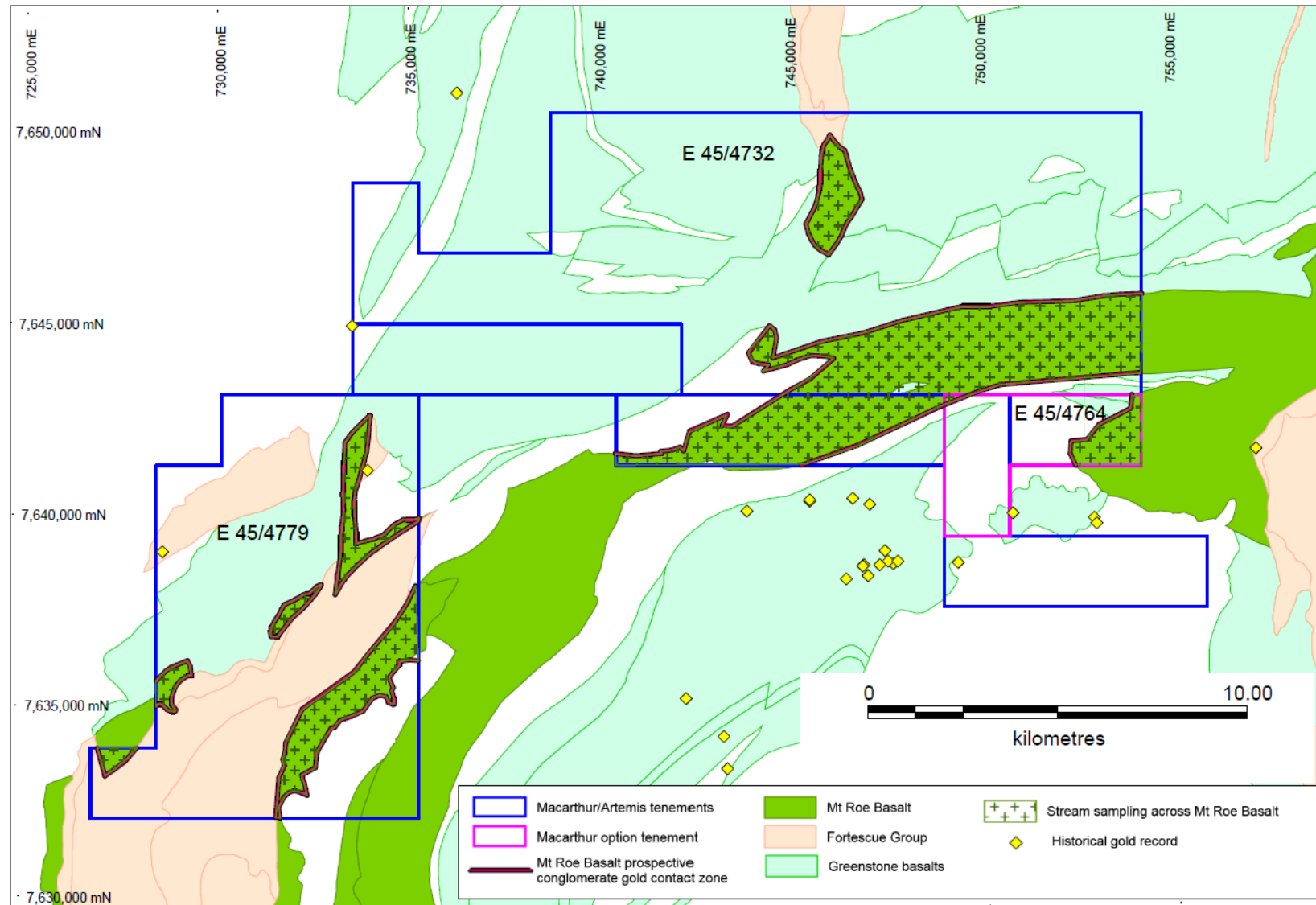
Figure 1. Macarthur Minerals' tenements showing area of interest for stream sediment sampling across the Mt Roe Basalt
