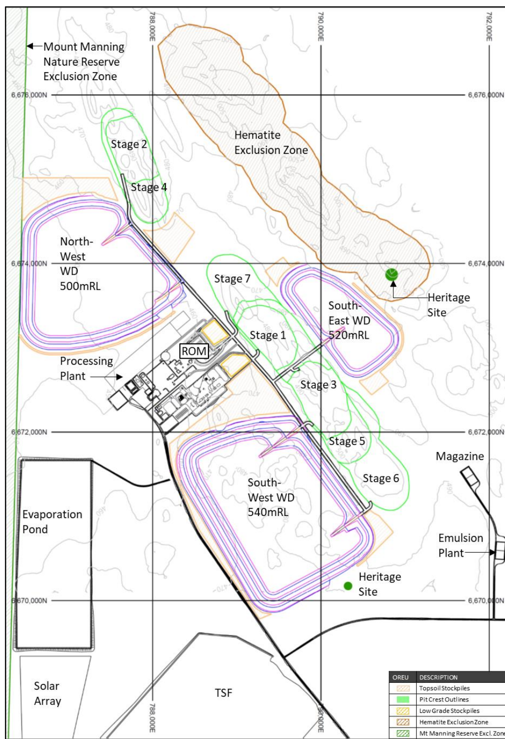
Figure 1 General site layout
